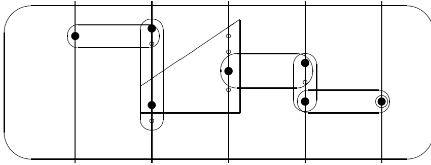
Fig. 6. Illustration for path l(x) D^{k<=}
