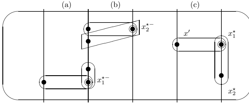
Fig. 4. Illustration for local and global optimum
