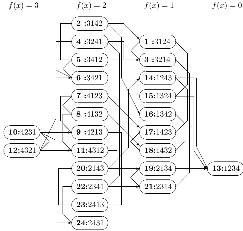
Fig. 2. Illustration for digraph D^{2\leq}
