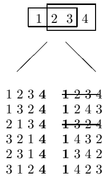
Fig. 3. Illustration for 3-neighborhood
