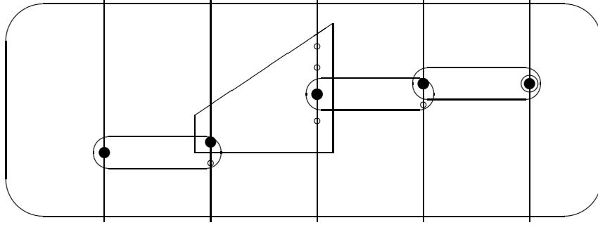
Fig. 5. Illustration for path l(x) D^{k<}
