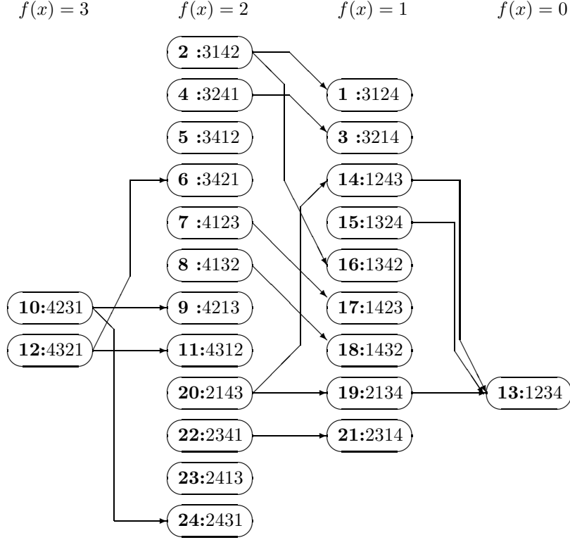
Fig. 1. Illustration for digraph D^{2<}
