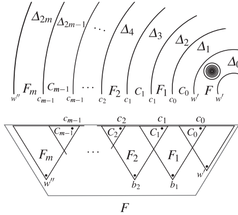
Figure 10: dd-morphism f , case (b4)
