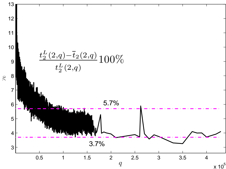
FIGURE 6. Differences in percentage between sizes t_2^L(2, q) of complete lexiarcs and the smallest known sizes \bar{t}_2(2, q) of complete arcs in \text{PG}(2, q)
