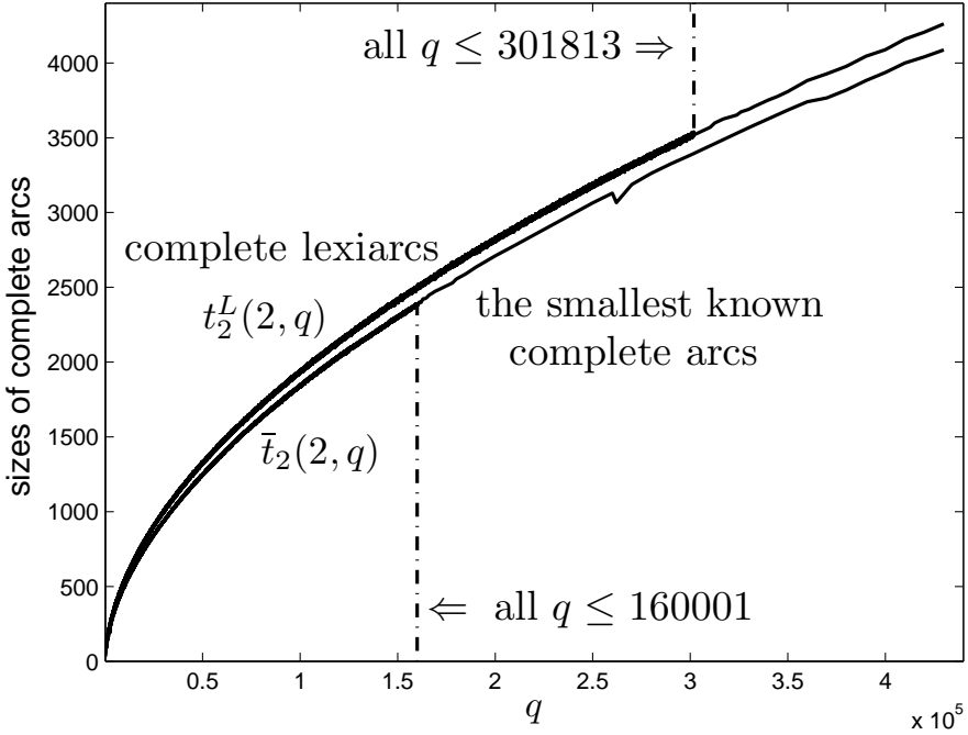
FIGURE 1. Sizes t_2^L(2, q) of complete lexiarcs in \text{PG}(2, q) , q \in L (top curve), the smallest known sizes \bar{t}_2(2, q) of complete arcs in \text{PG}(2, q) , q \in Q (bottom curve). Vertical lines mark regions of complete search for all q 's prime power.
