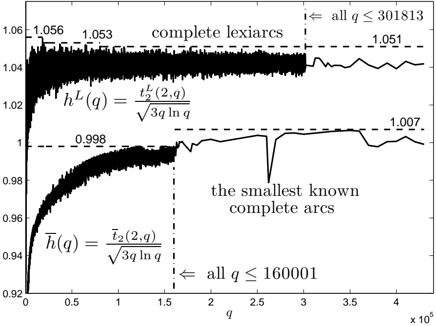
FIGURE 2. Values of h^L(q) = t_2^L(2, q) / \sqrt{3q \ln q} for complete lexiarcs in PG(2, q) , q \in L (top solid curve) and \bar{h}(q) = \bar{t}_2(2, q) / \sqrt{3q \ln q} for the smallest known complete arcs in PG(2, q) , q \in Q (bottom solid curve) and the corresponding upper bounds (dashed lines). Vertical lines mark regions of complete search for all q 's prime power.
