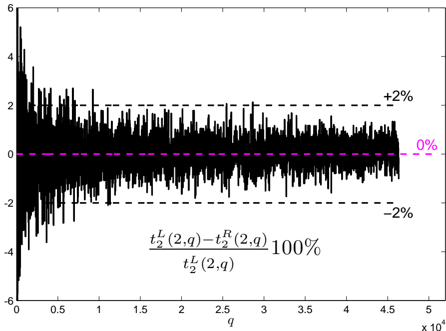
FIGURE 8. Differences in percentage between sizes t_2^L(2, q) of complete lexiarcs and sizes t_2^R(2, q) of random complete arcs in PG(2, q)
