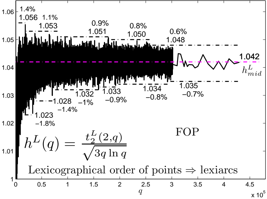
FIGURE 5. Values of h^L(q) = t_2^L(2, q)/\sqrt{3q \ln q} for complete lexiarcs in PG(2, q) , q \in L (solid curve) and the corresponding upper and lower bounds (dashed-dotted lines)
