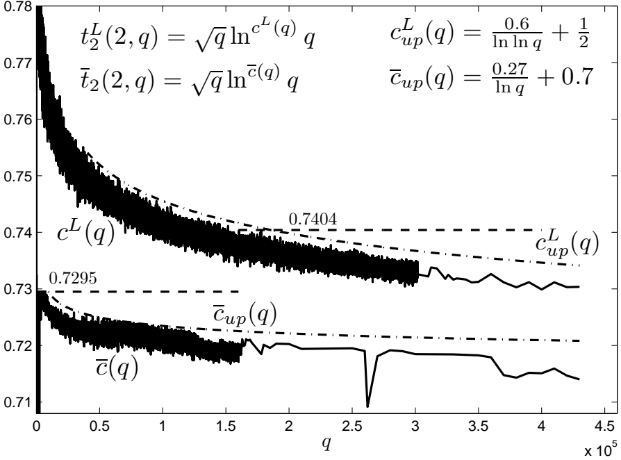
FIGURE 4. Values and bounds connected with decreasing function c(q) . Upper bounds “0.7404” and “0.7295” (dashed lines), upper bound c_{up}^L(q) = \frac{0.6}{\ln \ln q} + \frac{1}{2} (top dashed-dotted curve), values of c^L(q) for complete lexiarcs in \text{PG}(2, q) , q \in L (top solid curve), upper bound \bar{c}_{up}(q) = \frac{0.27}{\ln q} + 0.7 (bottom dashed-dotted curve), values of \bar{c}(q) for the smallest known complete arcs in \text{PG}(2, q) , q \in Q (bottom solid curve)
