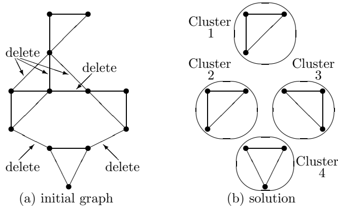
Fig. 5. Numerical example for balanced solution
